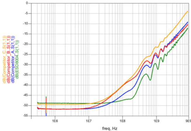
Figure 3. Return loss (S11) characteristics of ESD protection solutions
