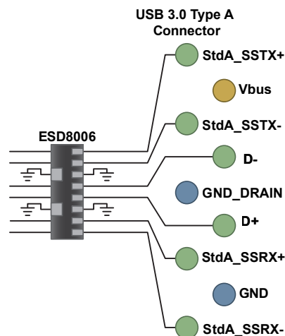
ESD8006 – 0.25 pF, 1 Layer Routing
